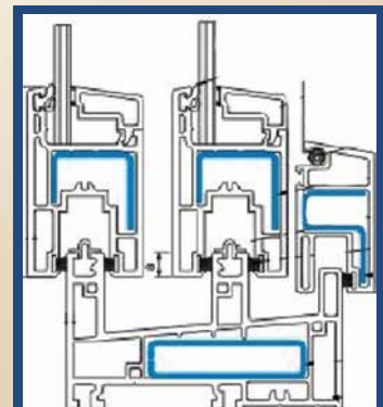
Sliding Window Line sketch
