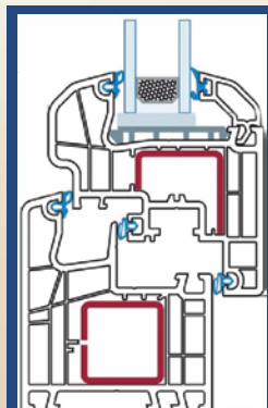
Openable window line Sketch
